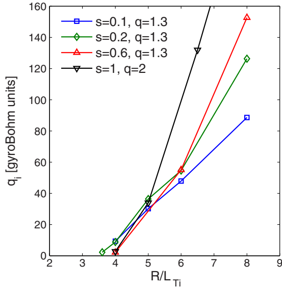
Figure 3. Nonlinear electrostatic collisionless GENE R/L_{Ti} scans for various levels of \hat{s} and q -profile with circular geometry at \rho = 0.33 . R/L_{Te} = 5 , and R/L_n = 1.1 .
